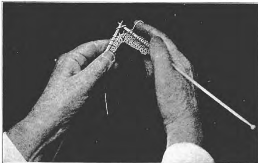
FIG. 2. POSITION OF HANDS IN PLAIN KNITTING
