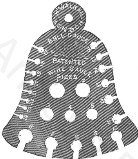
NO. 1.—WALKER'S BELL GAUGE.
